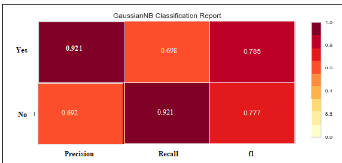
Figure 6-1: Performance matrix of the machine learning model
